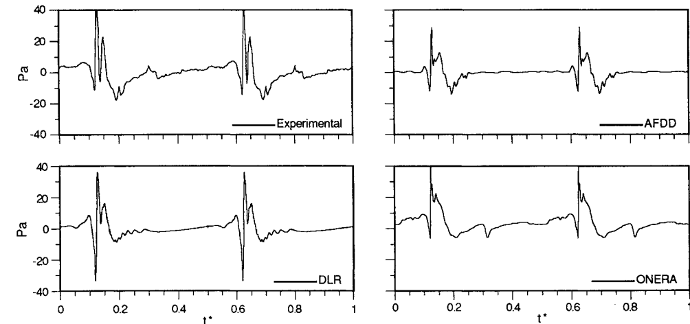
Fig. 9 OLS acoustic pressure time history at microphone 3 (run 10014 case).
