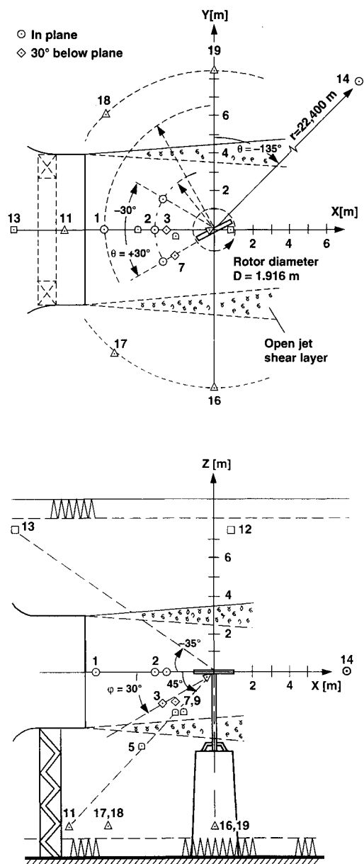
Fig. 2 Microphone locations in the DNW.
