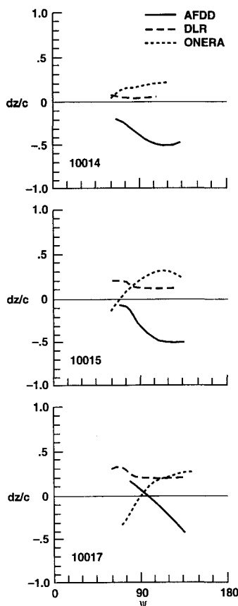
Fig. 4 Miss distances for a dominant interaction.
